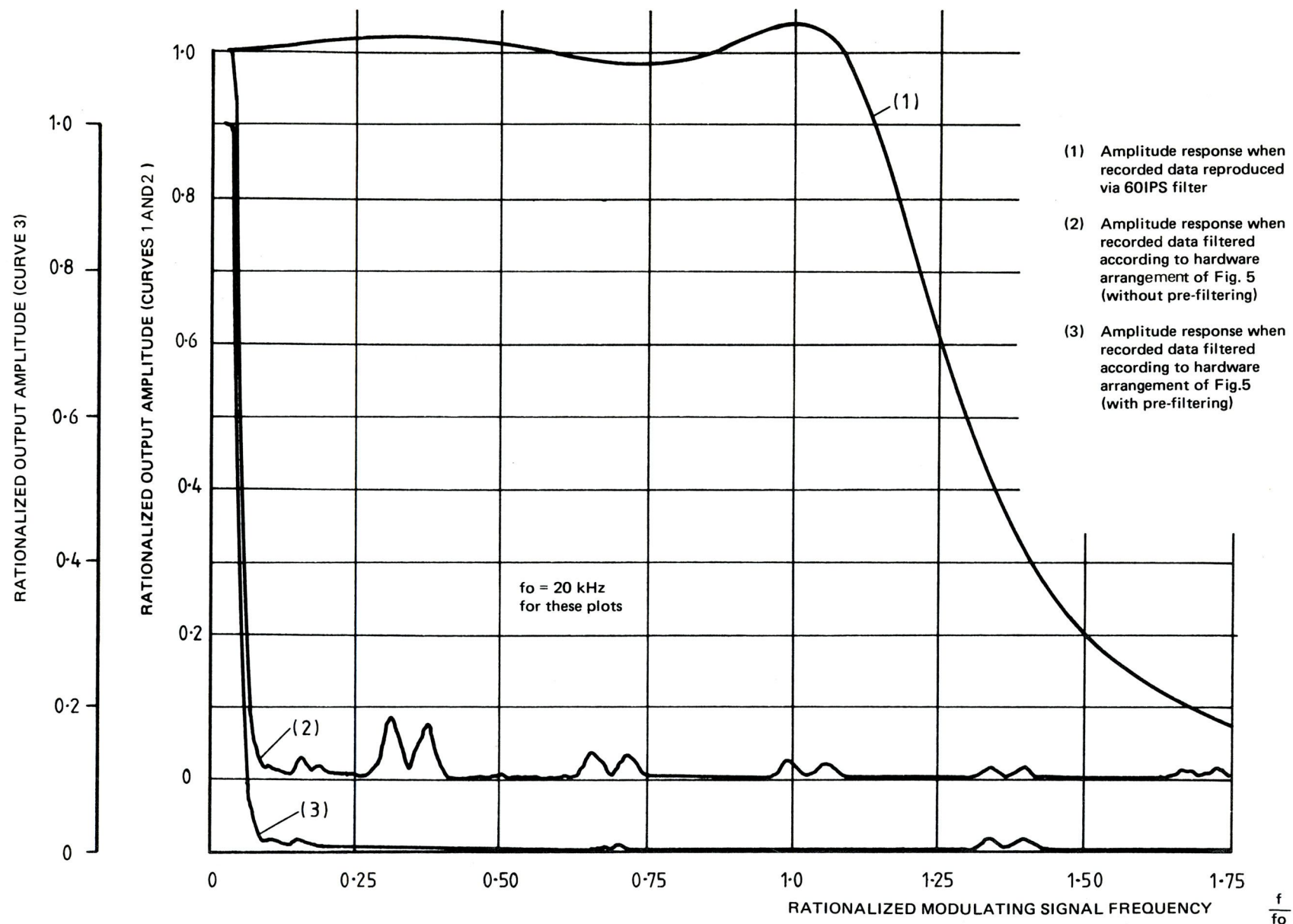
FIG. 6 REDUCTION OF SIDEBAND COMPONENTS WITH PRE-FILTERING
