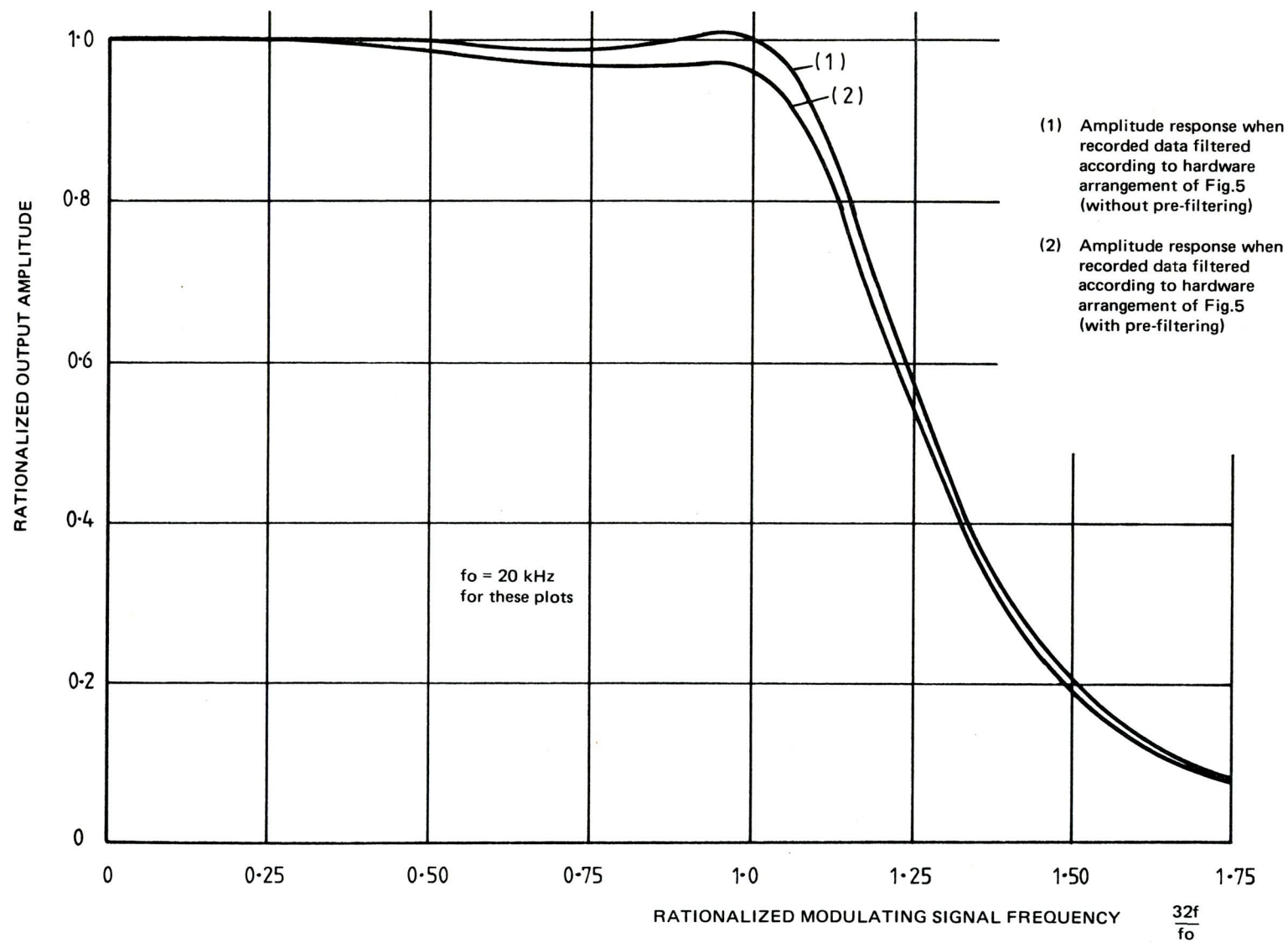
FIG. 7 EFFECT OF PRE-FILTERING ON LOW PASS FILTER AMPLITUDE RESPONSE
