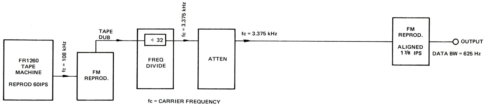
FIG. 5 (a) HARDWARE TO PRODUCE NORMAL FILTERING BUT WITH SIDEBAND NOISE
