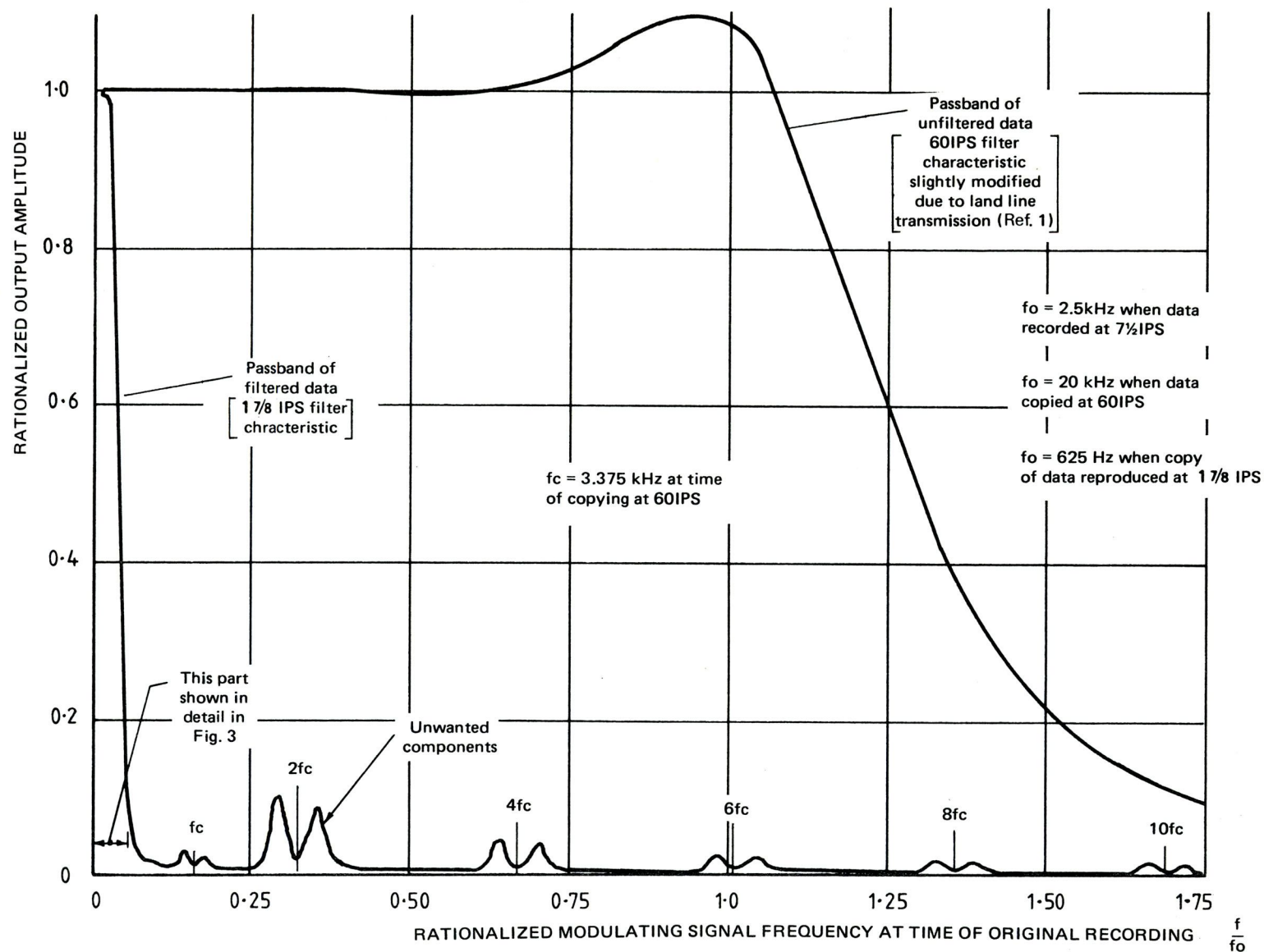
FIG. 2 COMPARISON OF FILTERED AND UN-FILTERED DATA PASSBANDS
