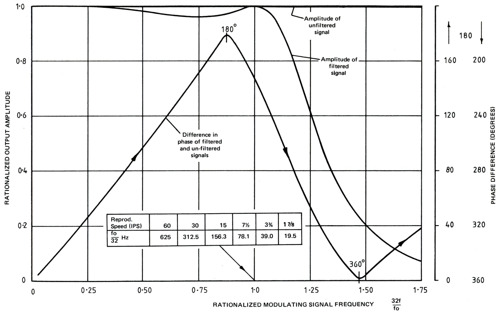
FIG. 3 AMPLITUDE AND PHASE RESPONSES OF LOW PASS FILTER
