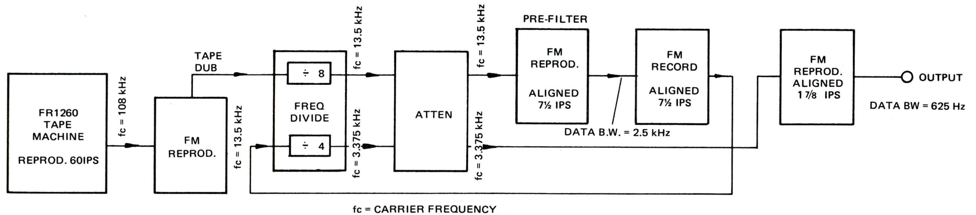
FIG. 5 (b) HARDWARE WHICH INCLUDES PRE-FILTER TO REDUCE SIDEBAND NOISE
